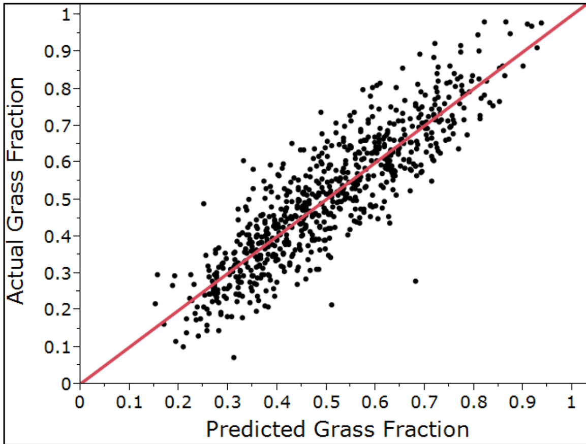
Figure 4 Actual versus model predicted values for the 2011 and 2012 sets from a candidate multivariate model (Table 4, Equation 30).
