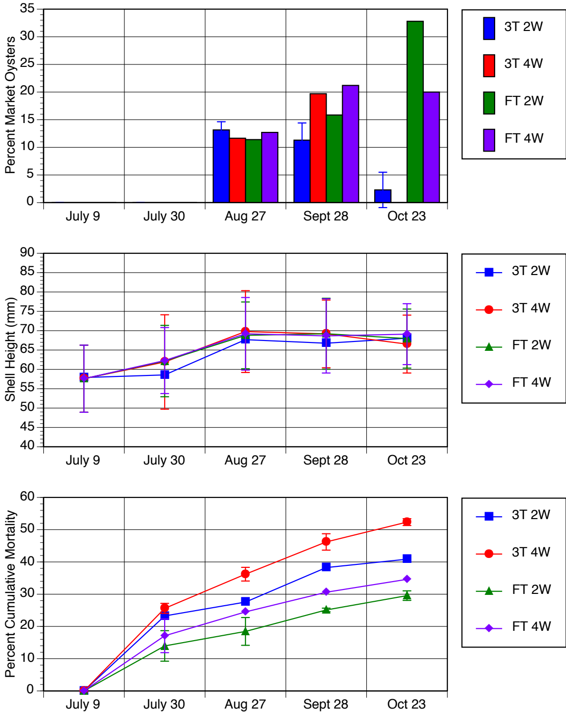
Figure 2. Percent market oysters harvested on each sample date (top), mean shell height (mm) (middle), and percent cumulative mortality (bottom) through time for the four treatment conditions: 3-tier cage with two week cleaning (3T 2W), 3-tier cage with four week cleaning (3T 4W), flip top cage with two week cleaning (FT 2W), and flip top cage with 4 week cleaning (FT4W). Error bars represent standard deviation.
