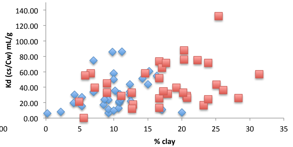
Kd vs. % clay
