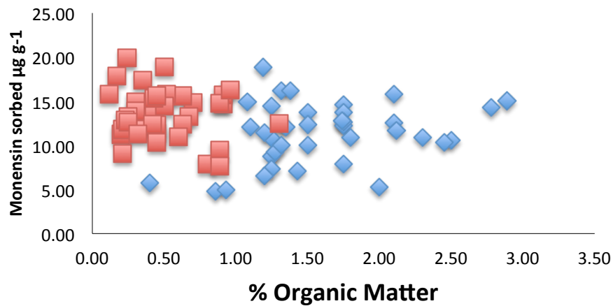
Sorption of Monensin vs. % Organic Matter
