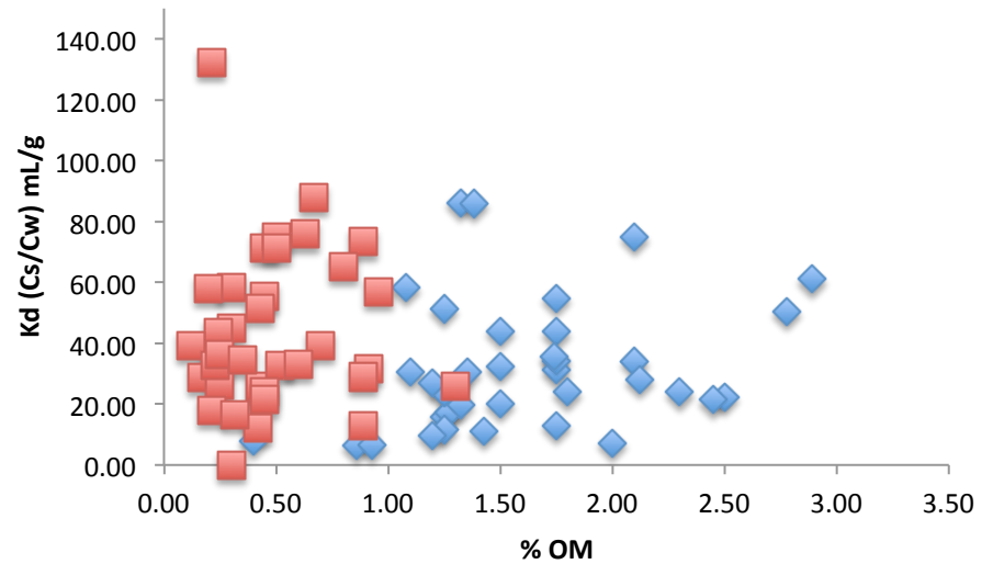
Kd vs. % Organic Matter
