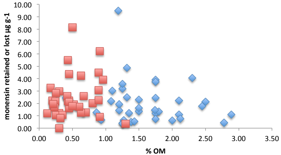
Hysteresis vs. % Organic Matter
