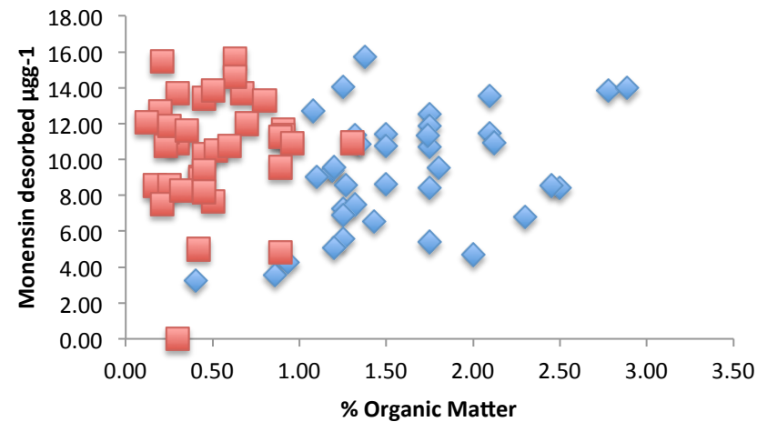
Desorption of Monensin vs. % Organic Matter
