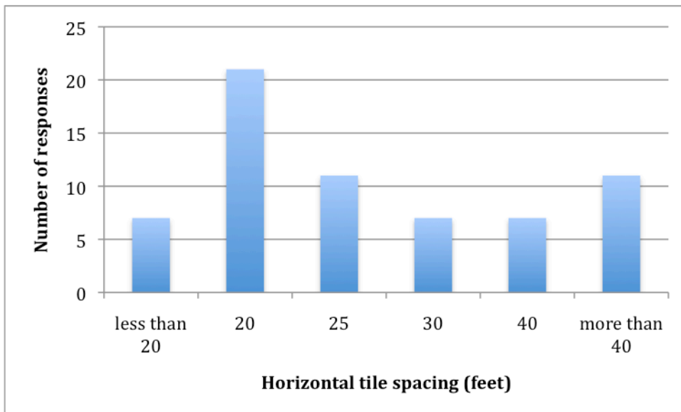
Figure 2. Range of responses to the question - "What is the horizontal spacing of your drain pipes?"
