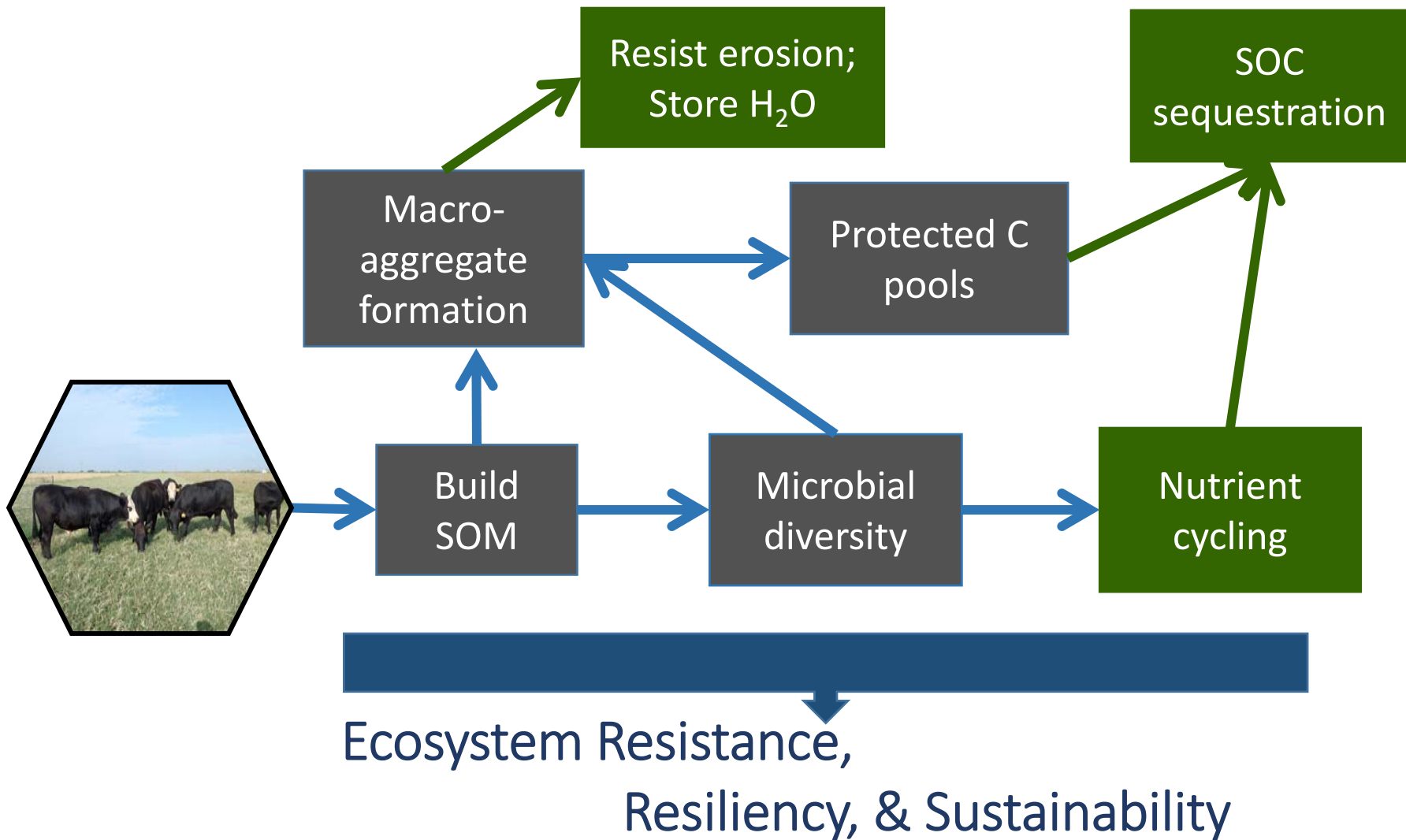
Fig. 10. Conceptual framework that depicts the major ecological benefits and mechanisms that impart these benefits as a result of integrated crop-livestock (ICL) agroecosystems in comparison to continuous cotton cropping systems (CTNc).
