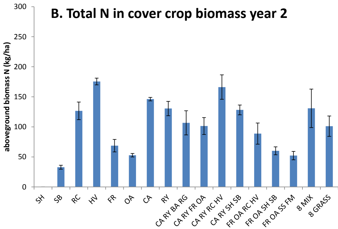
Figure 3. Total N retained in cover crop biomass in year 1 (A) and year 2 (B).
