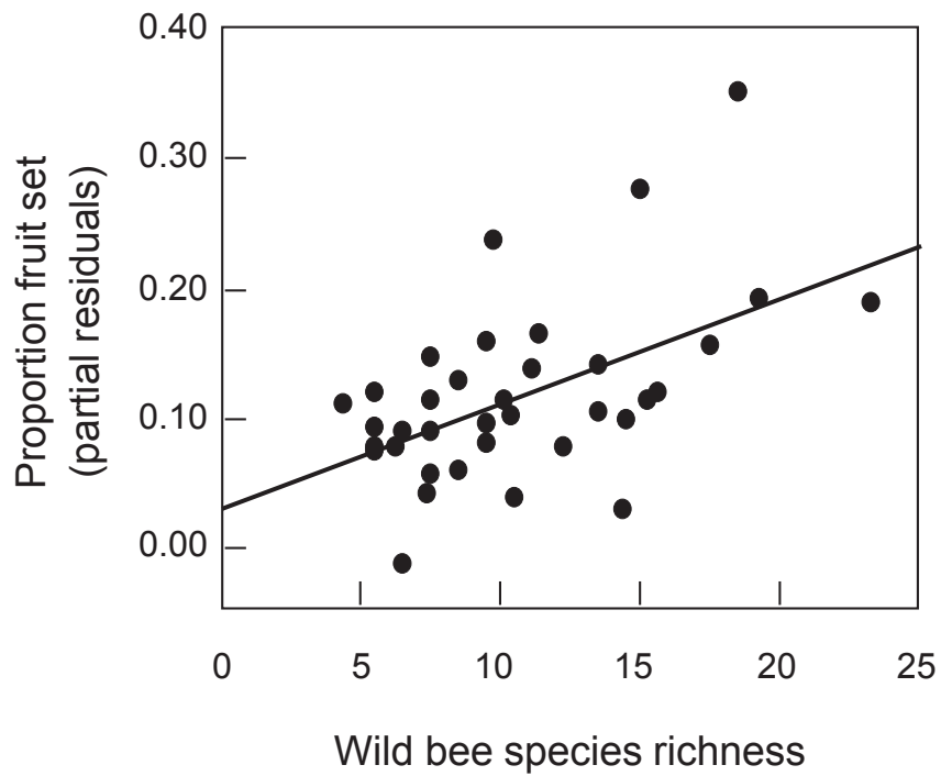
Figure 3. The effect of wild bee species richness on proportion fruit set after accounting for frost damage in a multiple regression model using data from 2012–2013.
