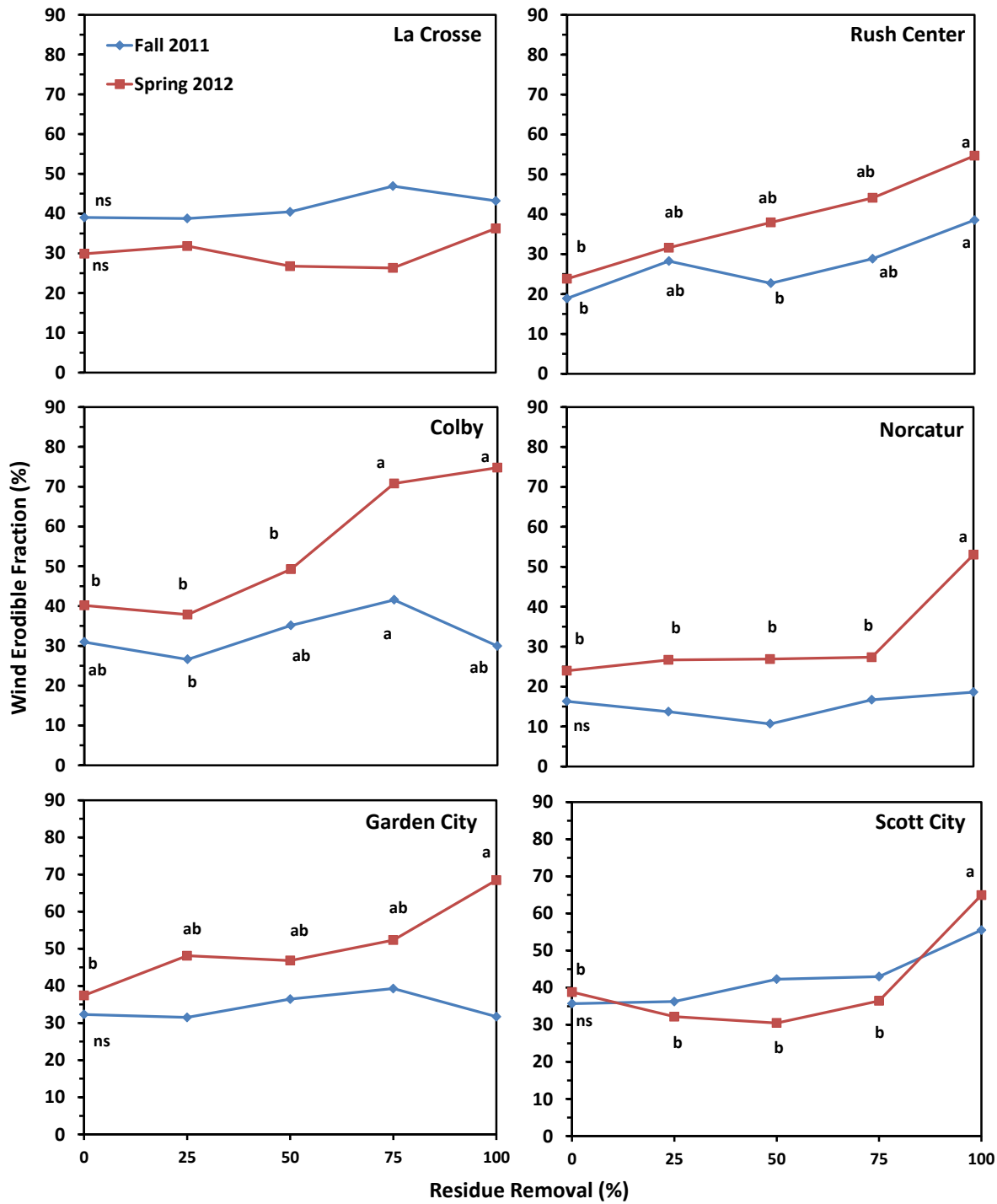
Figure. 3. Crop residue removal effect on wind erosion potential in Kansas.
