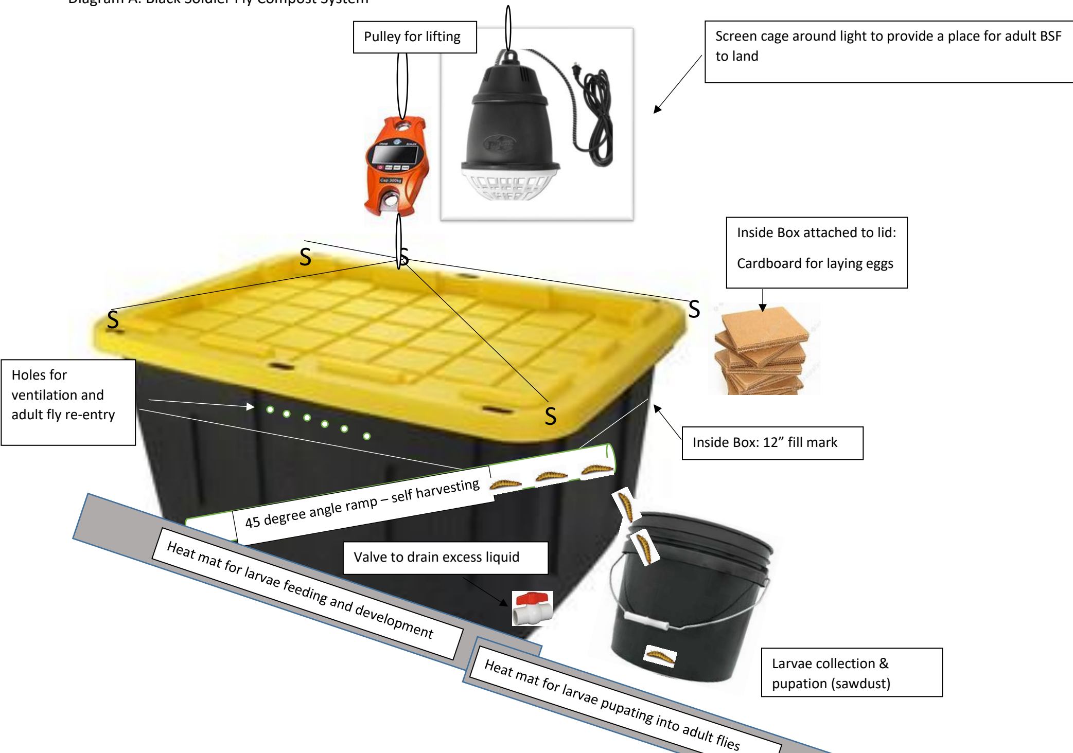
Diagram A: Black Soldier Fly Compost System
