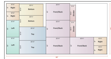
Figure 5. Barn owl nesting box board-cut template.
