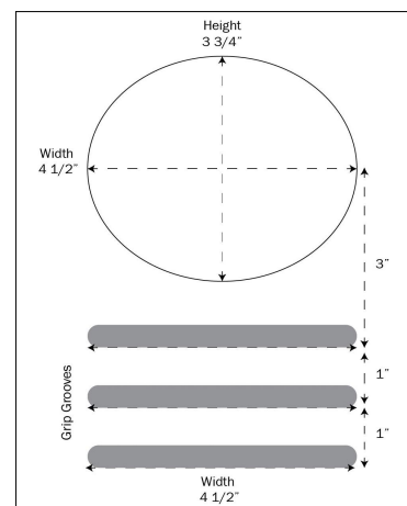
Figure 6. Entrance hole template.
