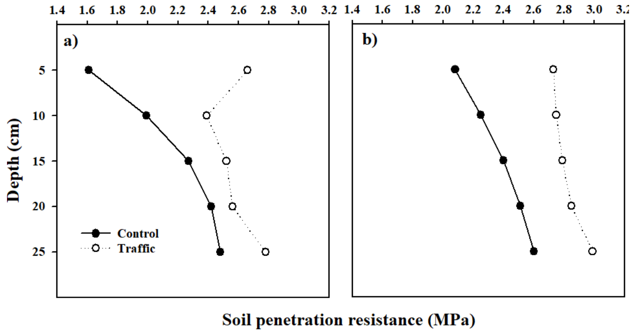
Fig. 1. Comparison of soil penetration resistance for control and trafficked rows during fall (a) and spring (b) at Freeman site.
