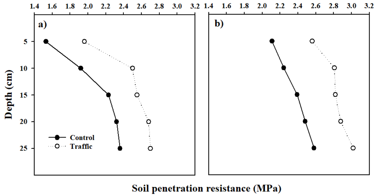
Fig. 2. Comparison of soil penetration resistance for control and trafficked rows during fall (a) and spring (b) at Plankinton site.
