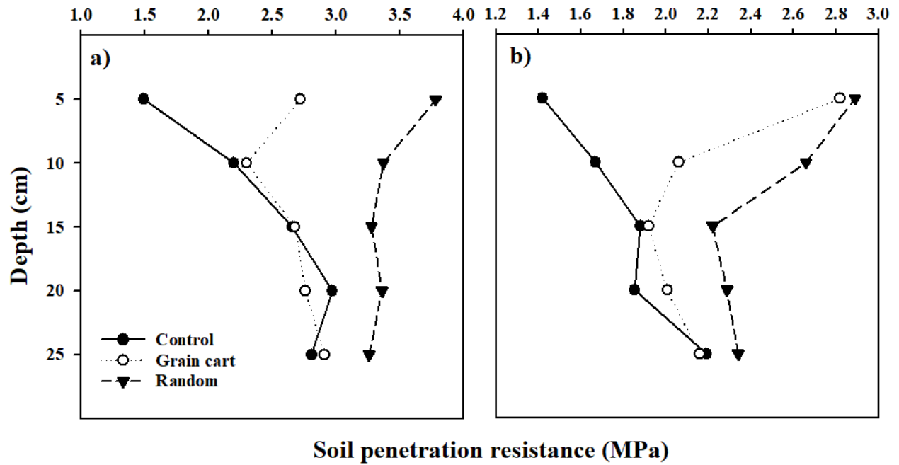
Fig. 3. Comparison of soil penetration resistance for single pass (a) and double pass (b) experiments at Gales Township site.
