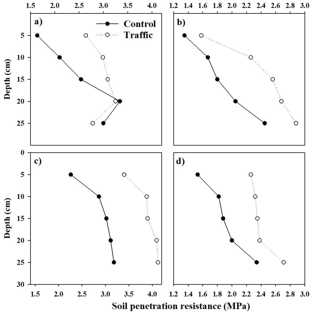
Fig. 4. Comparison of soil penetration resistance for control and trafficked rows at upslope (a) and (c) and downslope (b) and (d) at Red Rock site under the conventional tillage plots.
