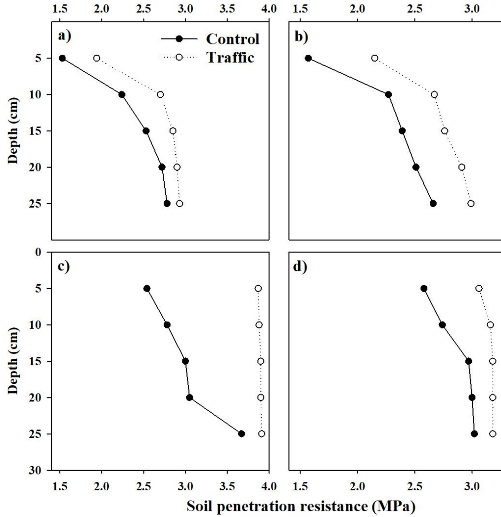
Fig. 5. Comparison of soil penetration resistance for control and trafficked rows at upslope (a) and (c) and downslope (b) and (d) at Red Rock site under the no-till plots.
