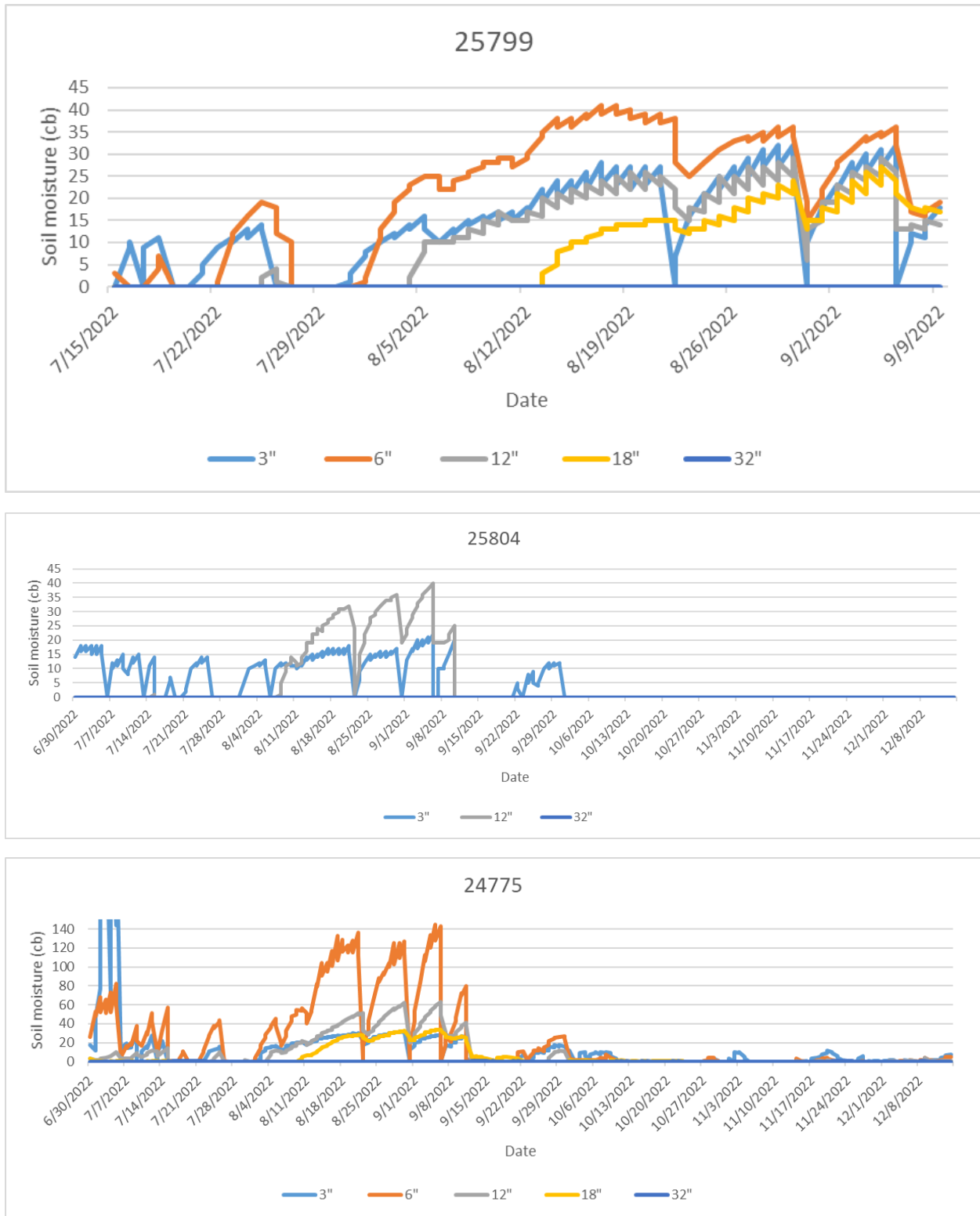
Figure 1. Soil moisture at three locations in the miscanthus field
