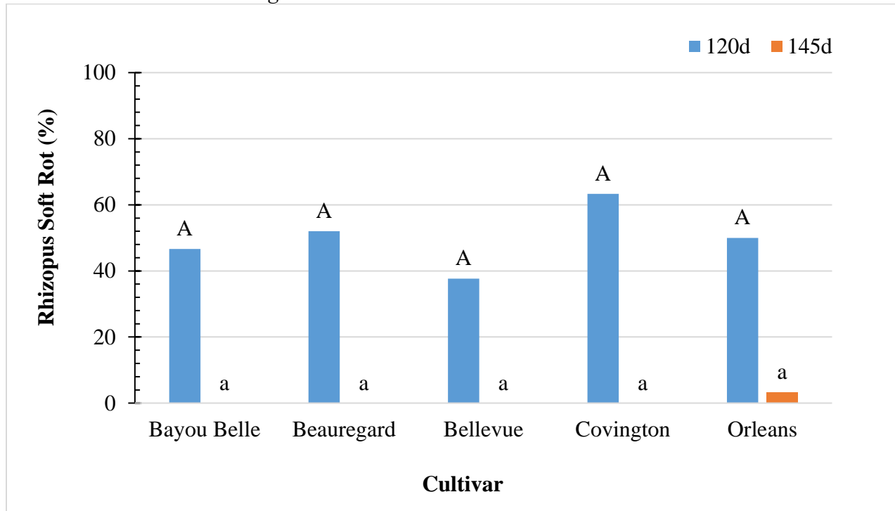
Figure 12. Effect of Bio-Save applied as spray on RSR incidence. Bars labelled with the same capital letter at 120 days or the same small letter at 145 days are not significantly different based on Fisher's LSD among odds at P < 0.05 .
