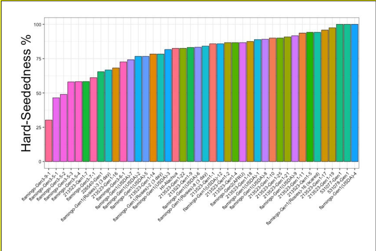
Figure 1. Variation in hard-seededness (%) present in hairy indigo germplasm after two runs of germination tests.
