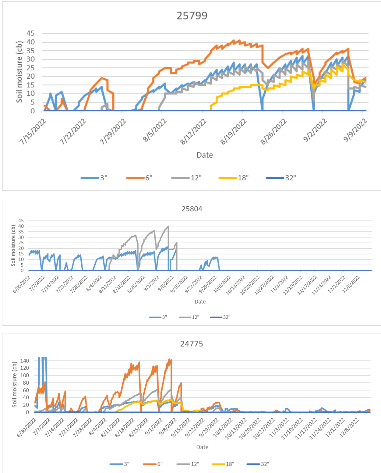
Figure 2. Soil moisture at three locations in the miscanthus field
