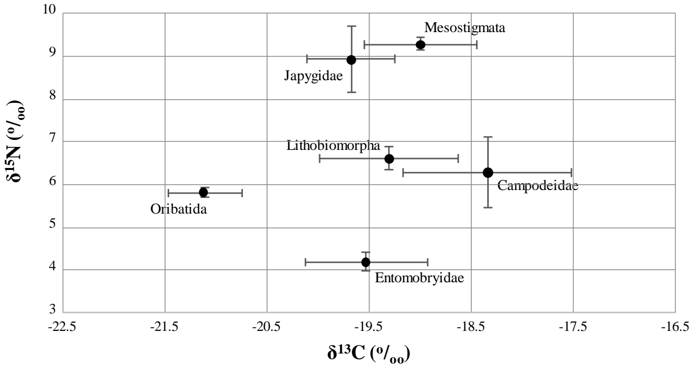
Figure 3. Mean ( \pm SE) values of the stable isotope signature for carbon ( \delta^{13}\text{C} ) and nitrogen ( \delta^{15}\text{N} ) measured in all soil fauna included in our analyses.
