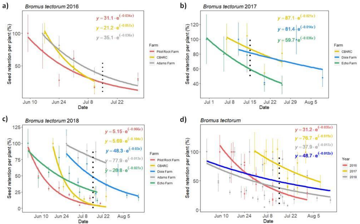
Figure 3. Seed retention per downy brome plant (%) in relation to calendar days in a) 2016, b) 2017, c) 2018, and d) all years. Parameters in equations indicate the percentage of seed retention on July 15 and the rate of seed shedding. Dotted vertical lines indicate July 15. Dots with symmetrical lines (standard errors) indicate experimental data and curves represent the fitted models. Dark blue curve in figure d indicates the average of the three years.
