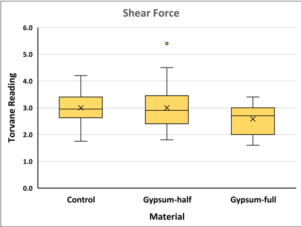
Figure 4. Boxplots of the effect of applied material on corn yield and relative shear force (Torvane reading) required to rupture crust 30DAE, 2021.
