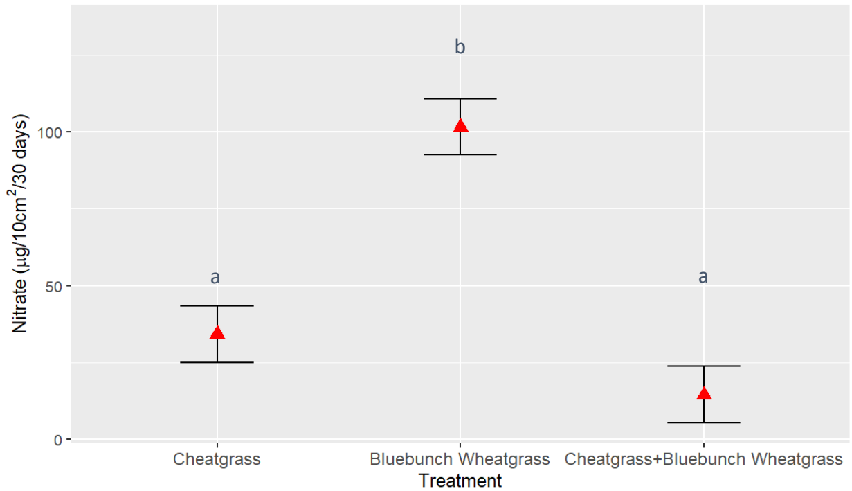
Figure 7: Available nitrate (NO 3 ) in pots containing cheatgrass alone, bluebunch wheatgrass alone, and cheatgrass and bluebunch wheatgrass grown together for 30 days in a greenhouse experiment. There was less nitrate available in pots containing cheatgrass. Triangles are the mean; error bars are constructed using standard errors. Species/treatments labeled with the same letter are not statistically different from one another using an alpha level of 0.05 and a Tukey's Honestly Significant Difference pairwise comparison test.
