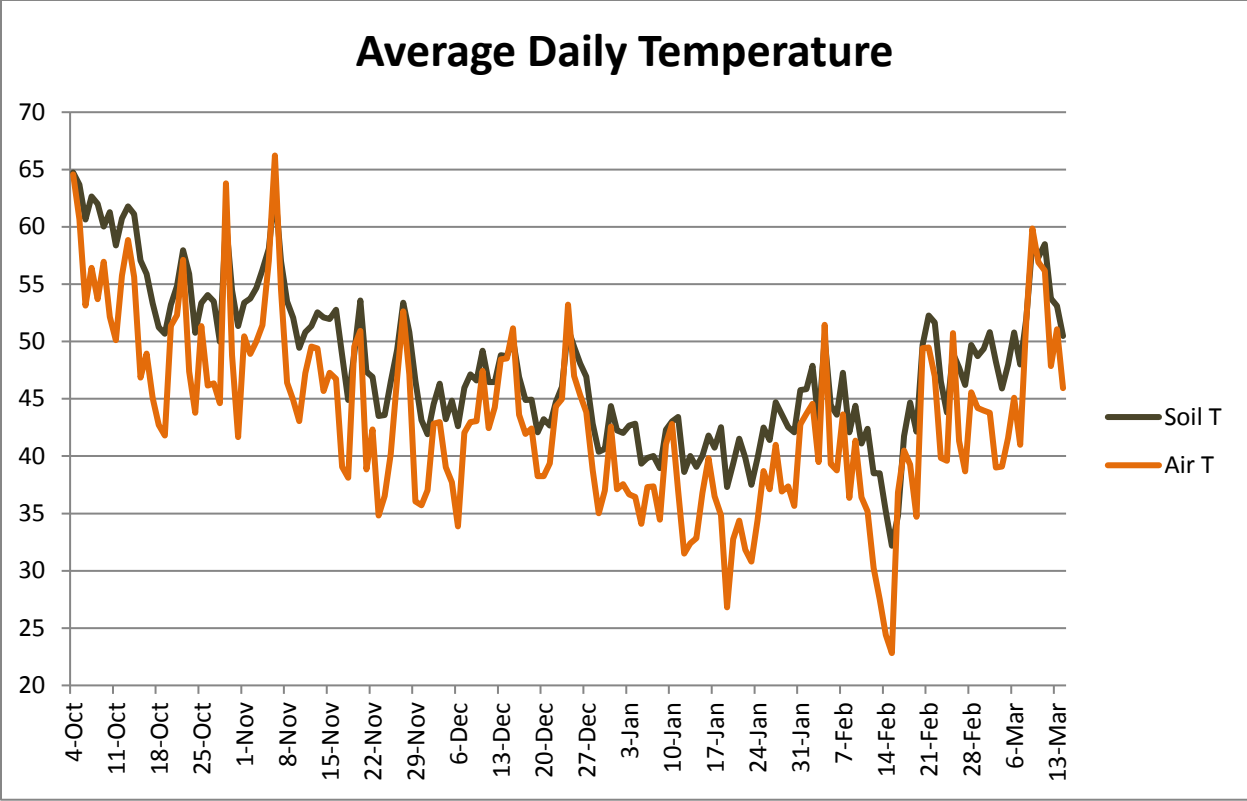
Figure 7. Average soil and air temperature in the tunnel shows that average soil temperature falls below 50F in early-November and, except for a few warm spikes, stays there until March.
