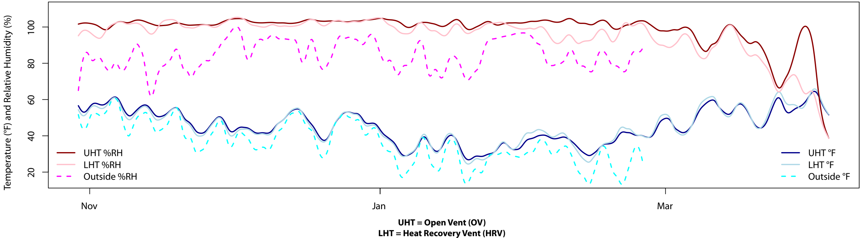
Temperature and Humidity Across All Three Treatments (Smoothed)
