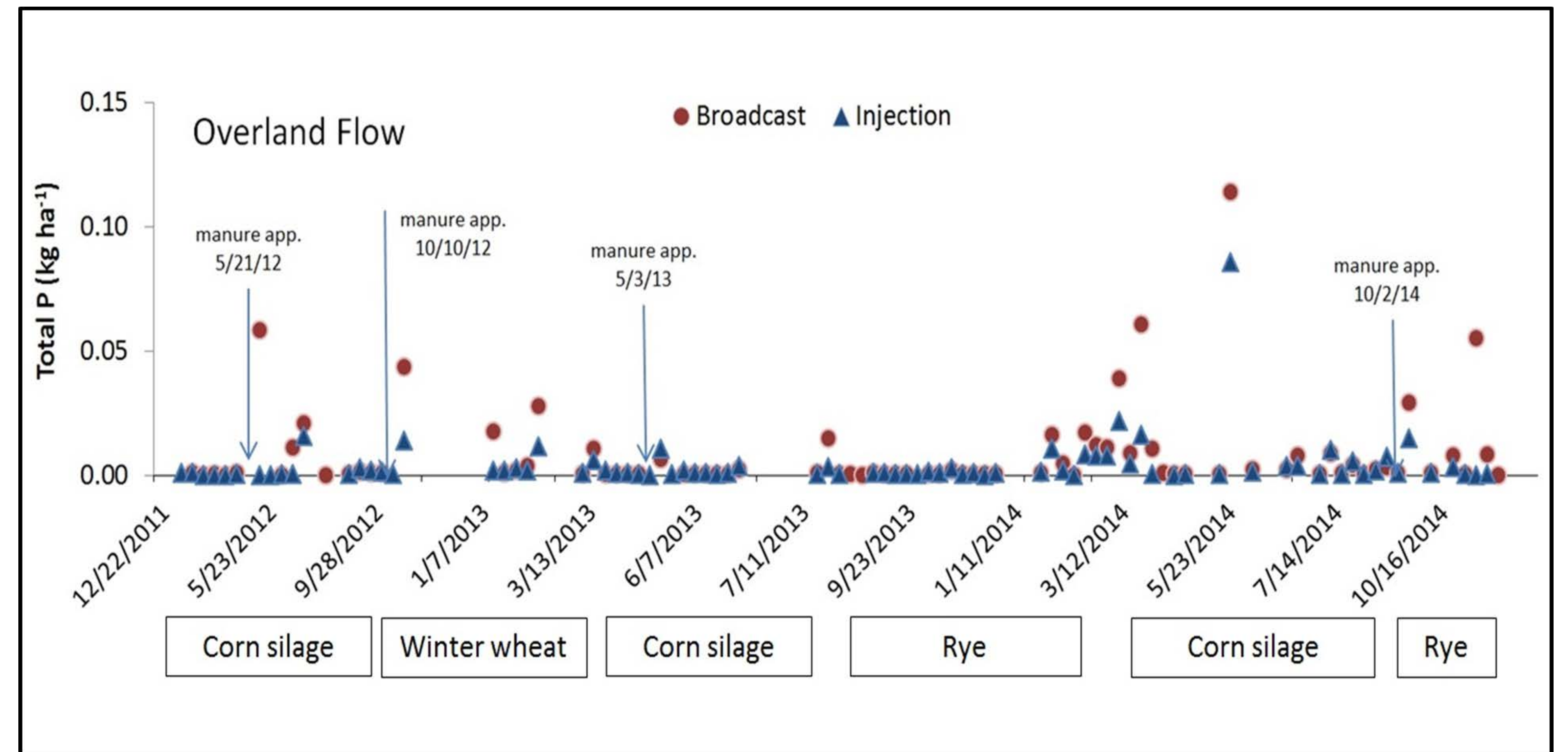
Total overland Phosphorus loss (kg/ha) averaged across manure broadcast and injection plots
