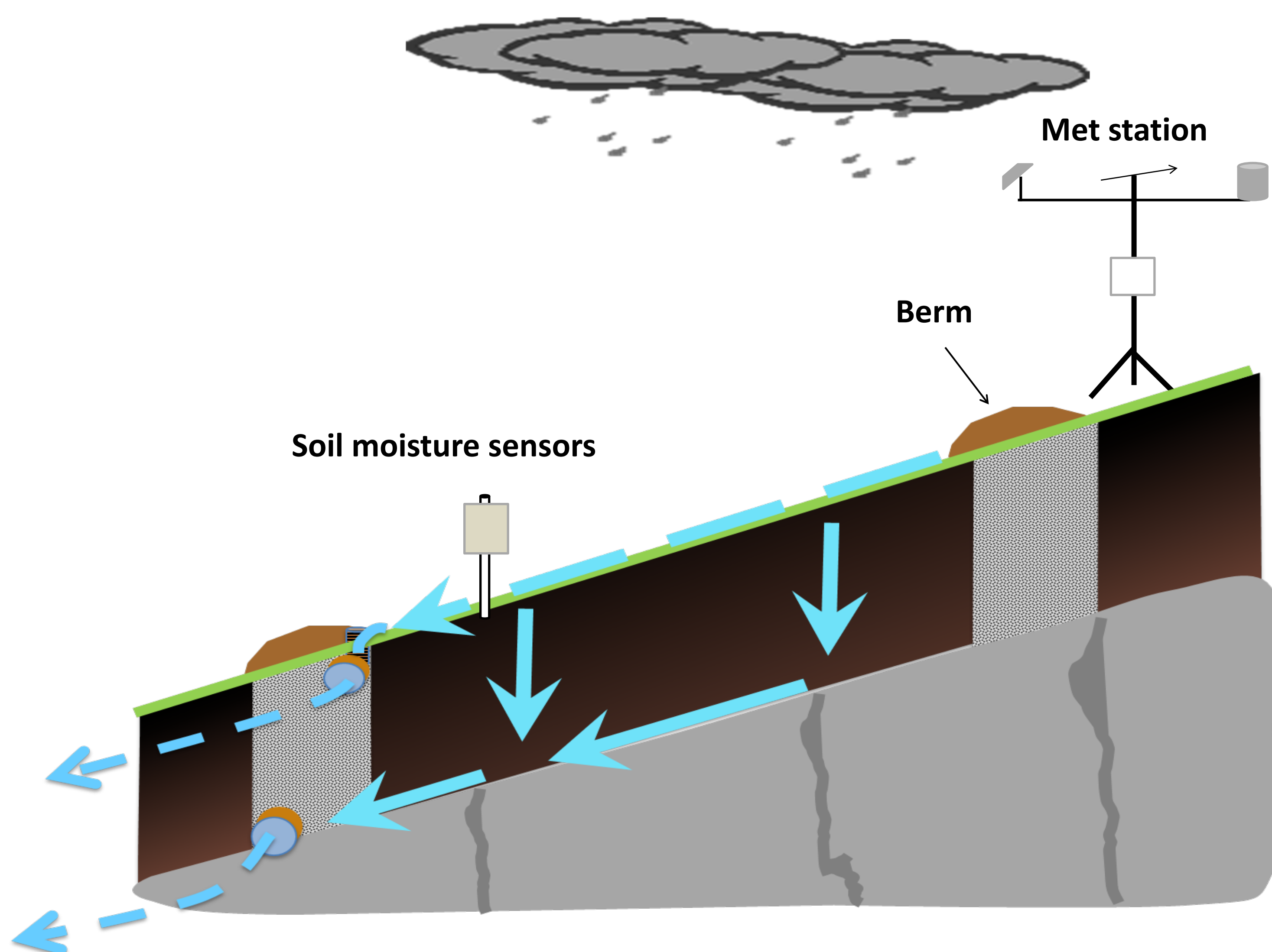
Leachate collection system and drainage at the representing plots
