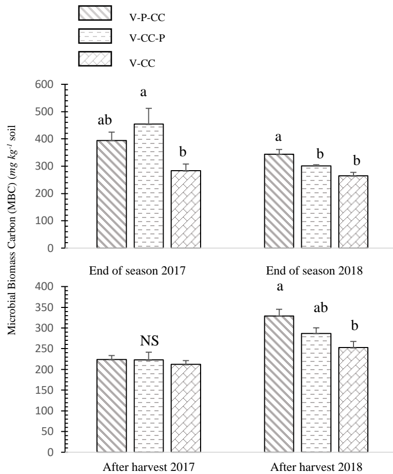
Figure 5. Microbial biomass carbon (MBC) at two sampling times; after harvest and end of season 2017 and 2018. Values with different letters are not significant between treatments within a given year at P < 0.05 .
