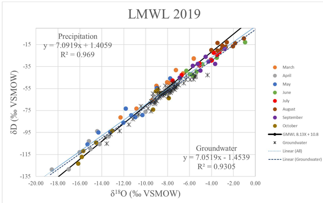
Figure 2. Local Meteoric Water Line generated using stable isotope composition of samples analyzed to date. The solid black line represents the Global Meteoric Water Line for reference. Groundwater data from a previous study are added for comparison.
