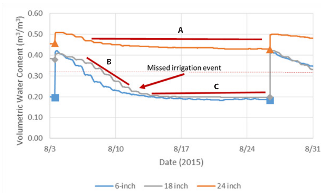
Figure 3. Example of soil moisture sensor data that depicts a missed irrigation event.
