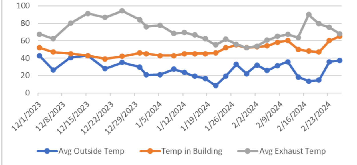
Temperature Graph- note avg 50kWh elec heat used 12/26 - 1/24
