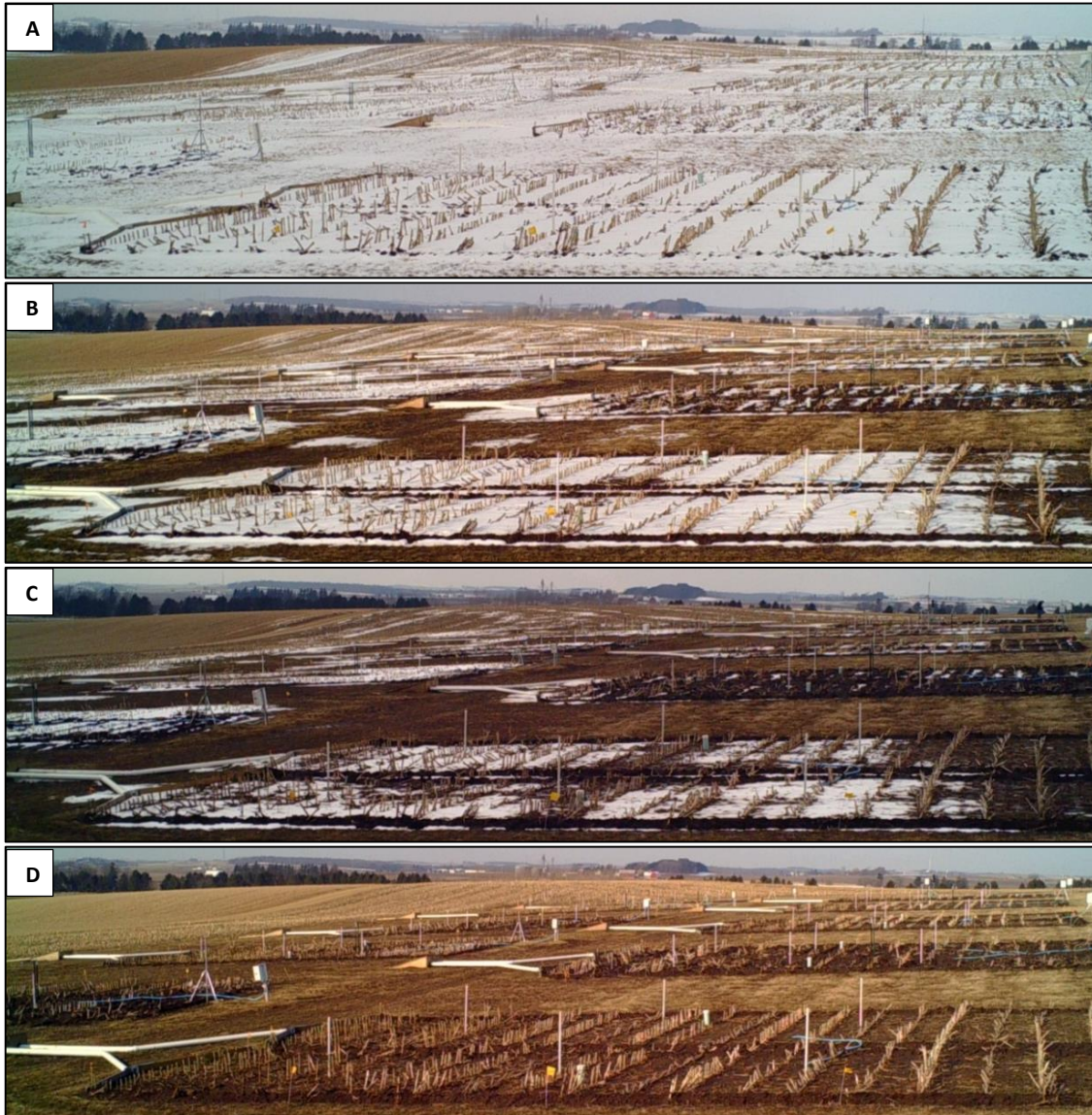
Figure 4. Time-lapse imagery of the plots during a period of thaw. A) 9:30 am on March 5, 2016, B) 2:30 pm on March 5, 2016, C) 1:00 pm on March 6, 2016, and D) 9:00 am on March 7, 2016.
