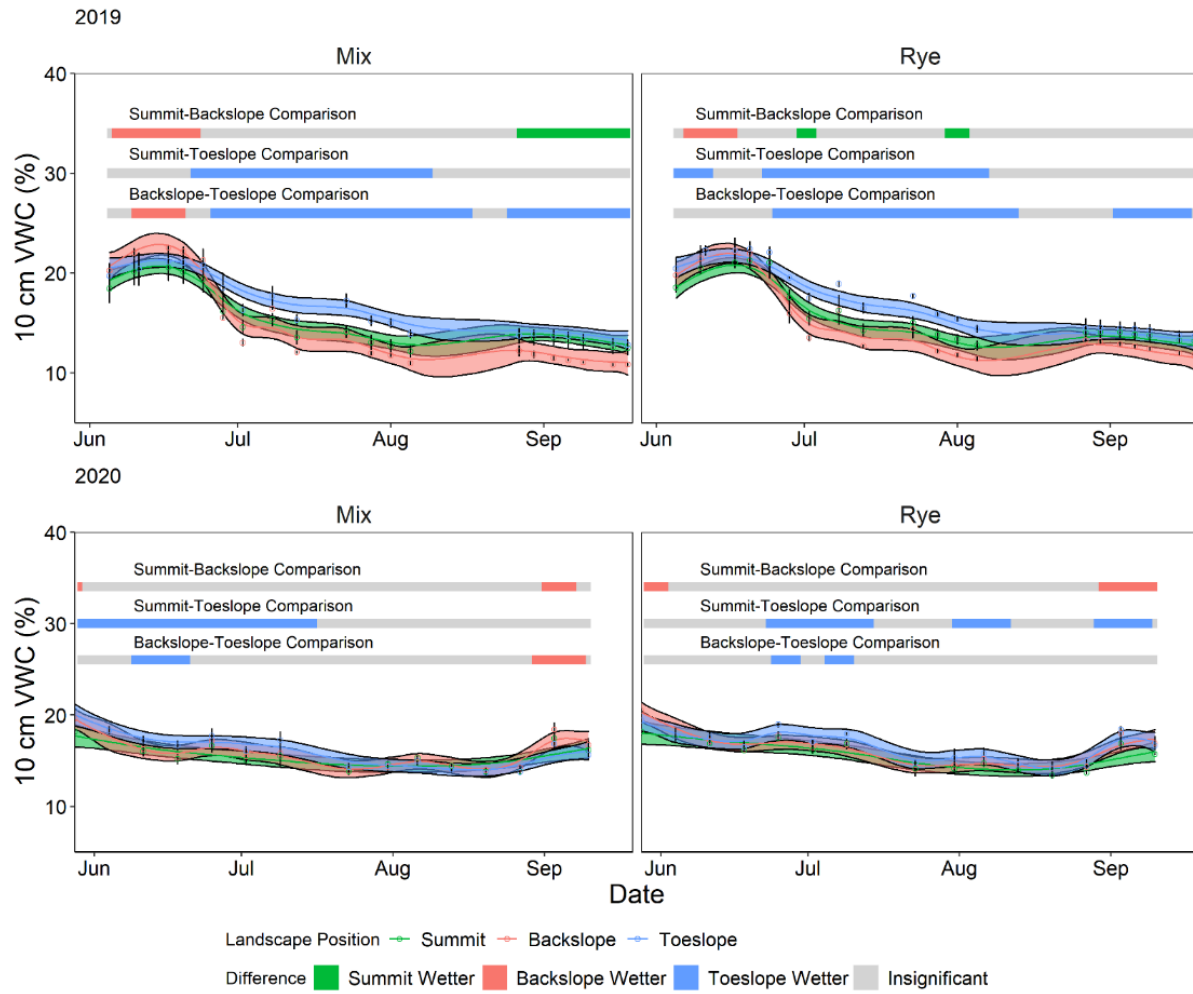
Figure 7 - Soil volumetric water (0-10 cm) taken weekly throughout the maize growing season for mixture (left) and rye (right) treatments, at each landscape position. The top panels reflect the 2019 growing season, the bottom panels reflect the 2020 growing season. Horizontal bars indicate the results of GAM analysis and indicate significant differences within a given pairwise comparison. Ribbons surrounding the predictions indicate the 90% confidence interval. The points indicate the average of three measurements on each sampling date, error bars are +/- 1 SE.
