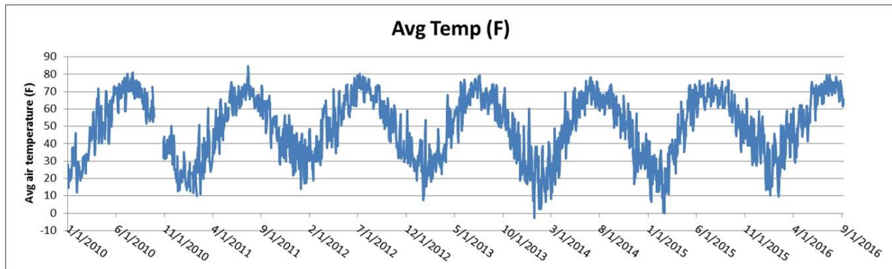
Figure 2. PSU NESARE dairy cropping systems daily average air temperature (in) (2010-2016). Weather data were collected from 2010 to 2016 at the Natural Resources Conservation Service (NRCS) weather station site at Rock Springs, Centre County, Pennsylvania (40°43' N; 77°56' W, 1220 feet elevation) and the weather station at our lysimeter plots.
