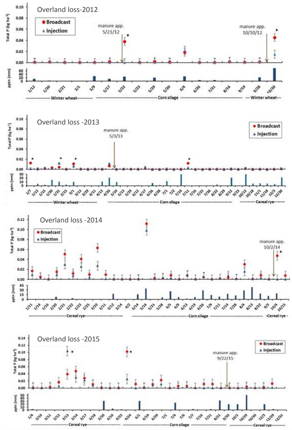
Figure 3. Total overland P loss (kg ha -1 ) from lysimeter plots (2012-15). * indicates significant difference at P \leq 0.01 .
