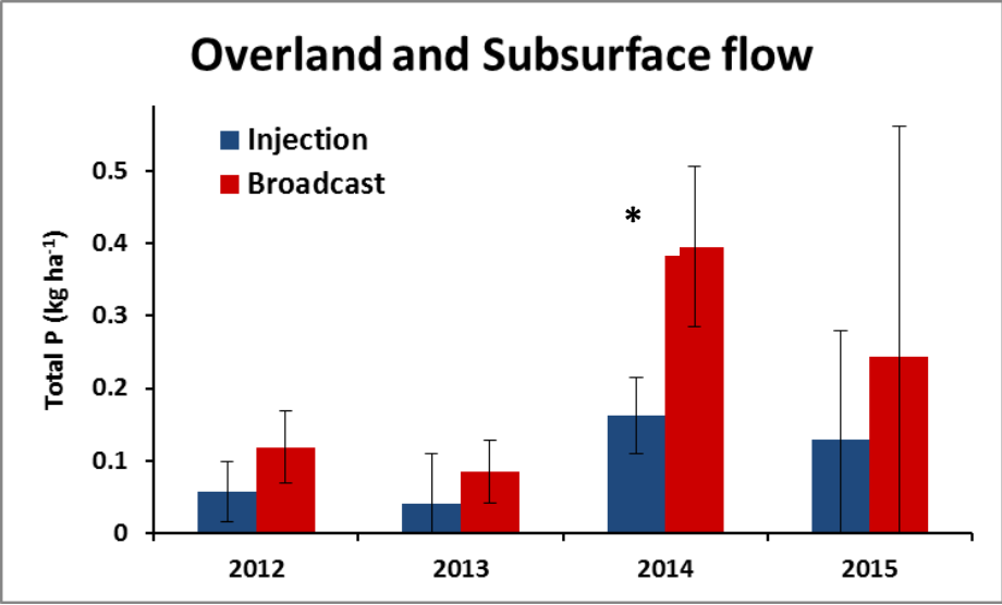
Figure 6. Total annual P loss in both overland and subsurface flows. Bars are standard error.
