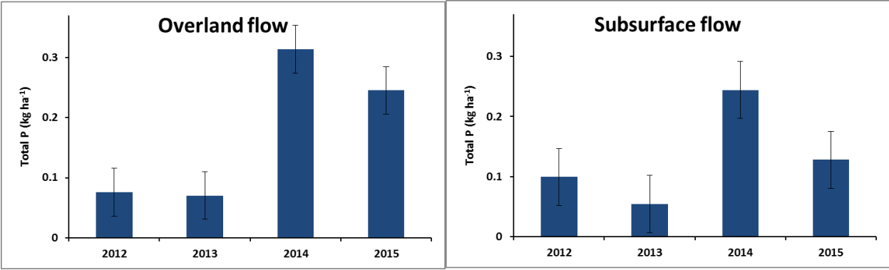
Figure 5. Total annual P loss in the overland and subsurface flows. Bars are standard error.
