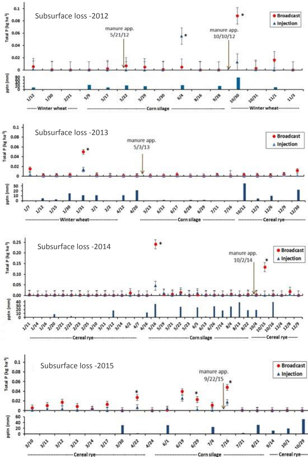
Figure 4. Total subsurface P loss (kg ha -1 ) from lysimeter plots (2012-15). * indicates significant difference at P \leq 0.01 .
