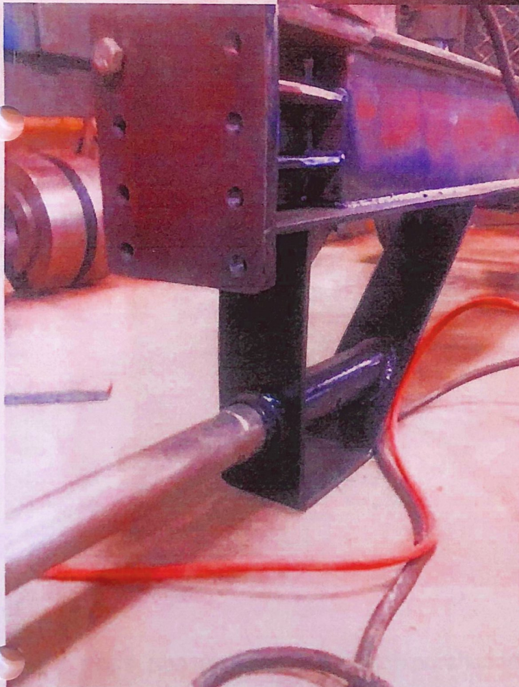
3. Support foot for operating end of the unit. ( 3/8 "x 4-1/2 " plate bent into foot. Fitted with 2-1/2 " pipe receiver for the removable tongue assembly. ( 2 " pipe with hitch welded on end for 1-7/8 ball hitch.)
